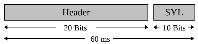
Figure A.2.6-1: Construction of the IS_SYL Message
