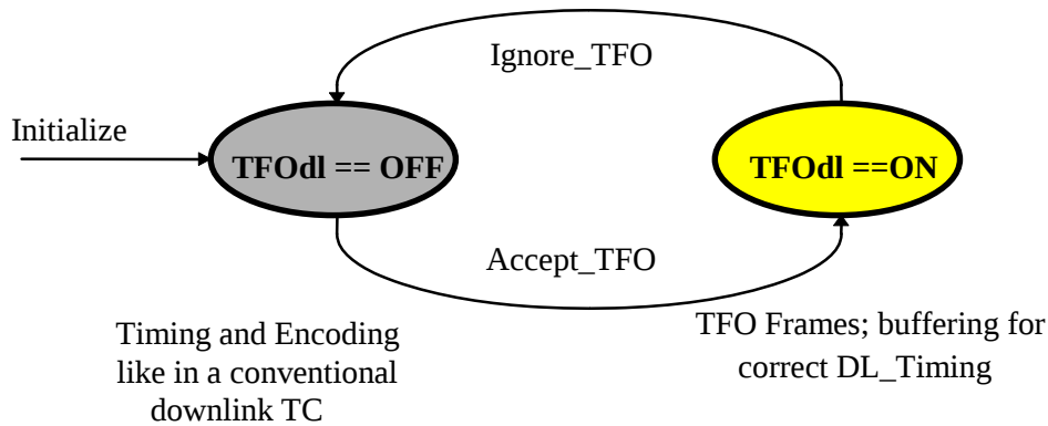
Figure D.3.2-1: States of the Tx_IU Process
