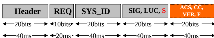
Figure 7.11.3.1-1: Construction of the shortest possible TFO_REQ Message for any AMR Codec Type
