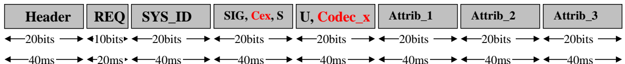
Figure 7.4-3: Example of a TFO_REQ Message with a Codec with an index higher than 15 and with three Attribute Extension_Blocks (300 ms length)
