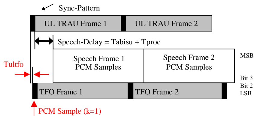
Figure 8.1.2-1: Uplink TFO Frame Time Alignment in GSM
