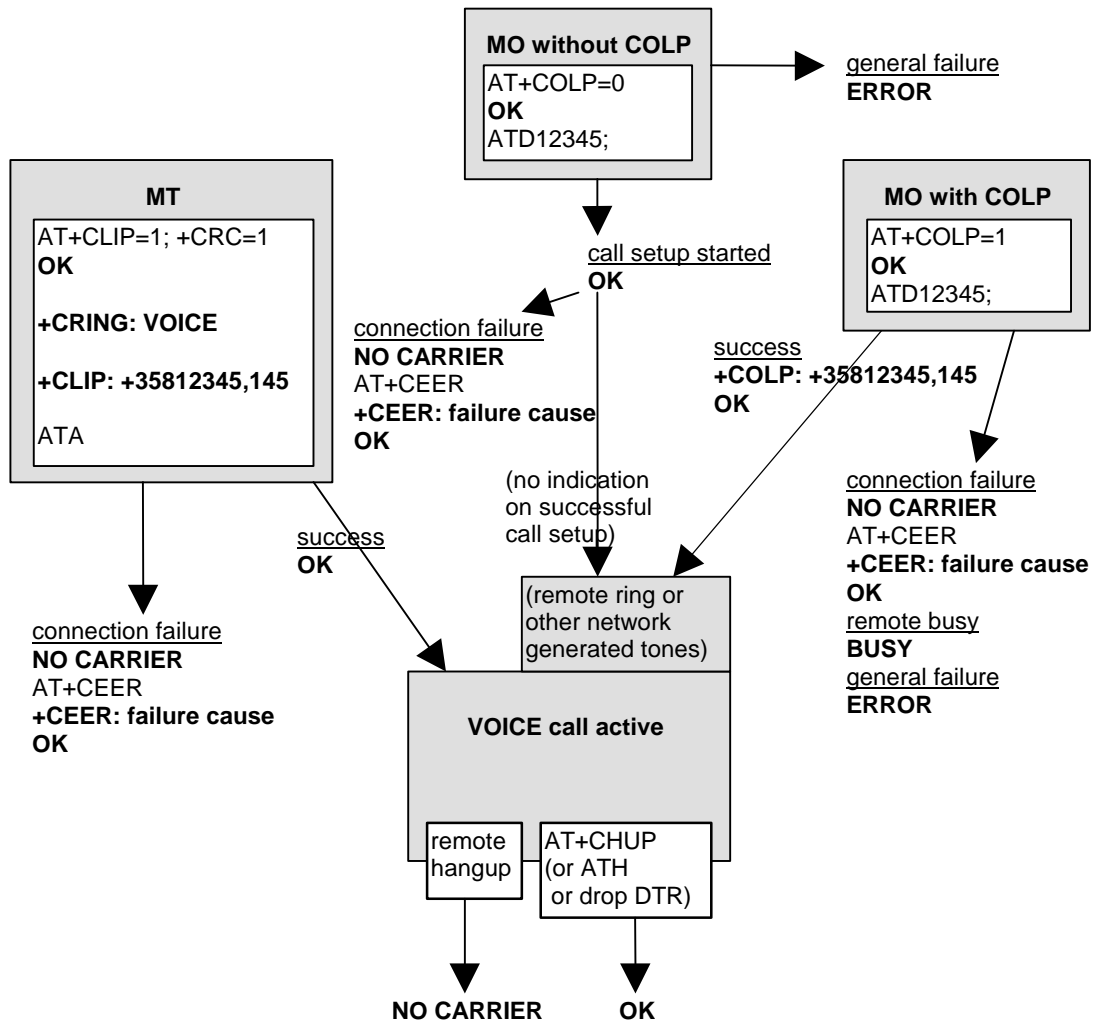
Figure G.1 illustrates the possible transitions in both MT and MO TS 11 calls. Responses and result codes generated by TA are in bold face.
