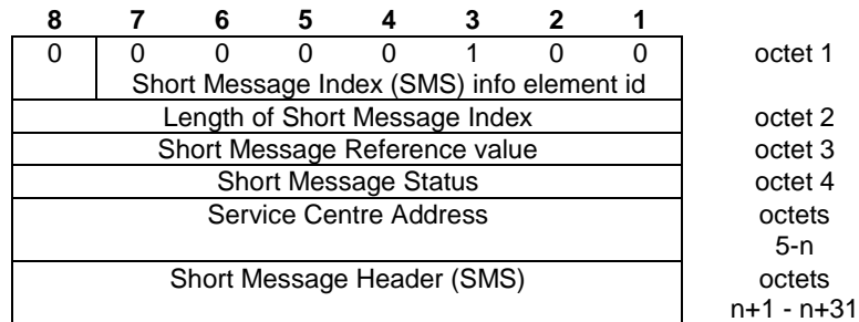
Figure 2.5.6: Short Message Index (SMS) information element
