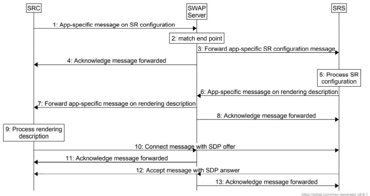
Figure 8.2-1 Call flows for SWAP message exchange
