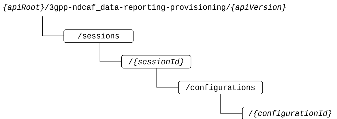
Figure 6.2.1-1: URL path model of Ndcap_DataReportingProvisioning service API
