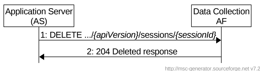
Figure 4.2.5.4-1: Application Server destroys DataReportingSession
