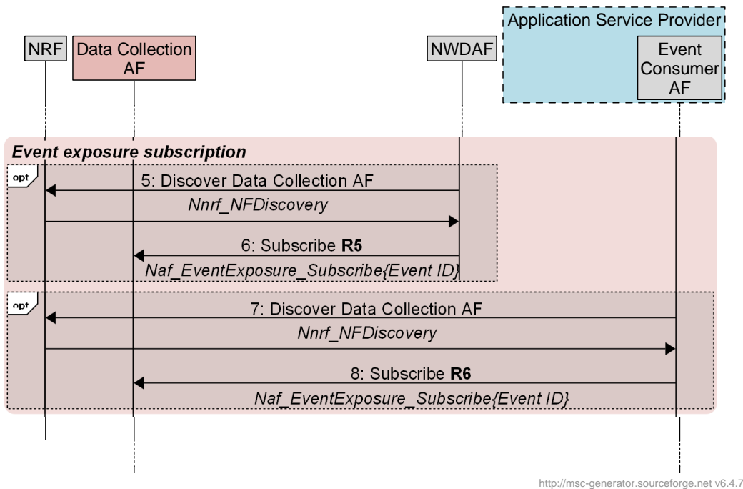
Figure 5.3-1: High-level procedures for subscription phase
