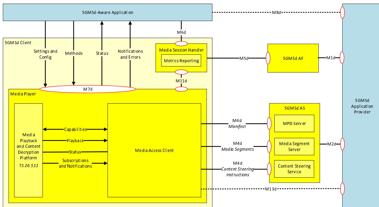
Figure 10.2-1: M4d usage for DASH distribution
