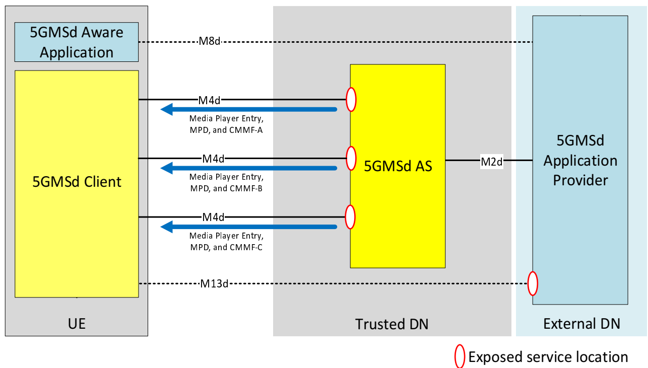
Figure H.3.3.2.1-1: Basic deployment example for 5GMSd AS ingest, content preparation, and delivery using CMMF
