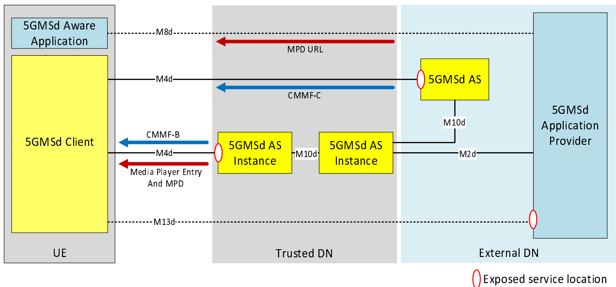
Figure H.3.3.3.1-1: Centralized 5GMSd AS content preparation and ingest deployment example
