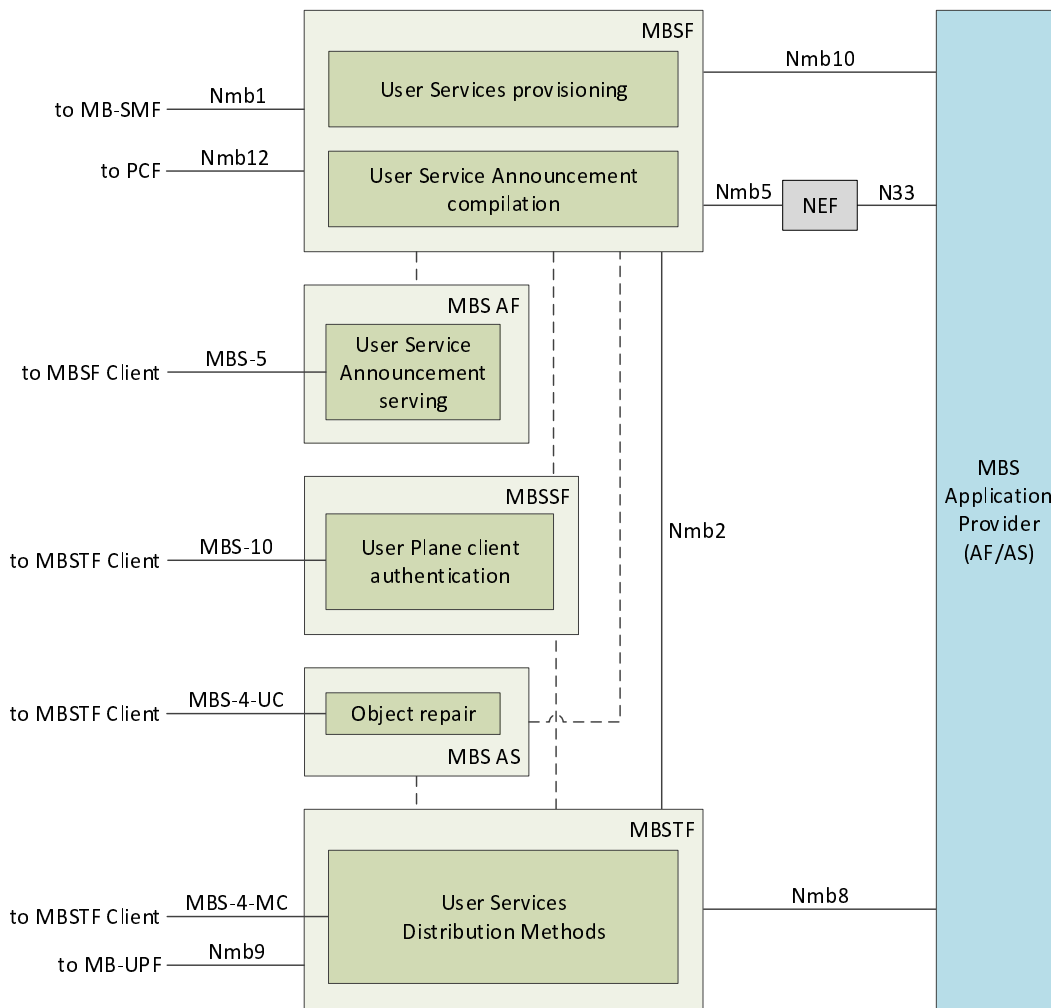
MBS User Services network architecture
