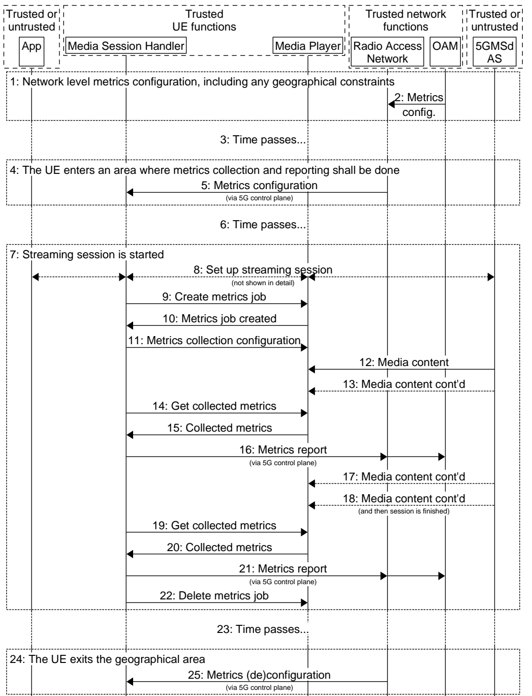
Figure 5.5.2-1: Metrics collection using the out-of-band 5G control plane option
