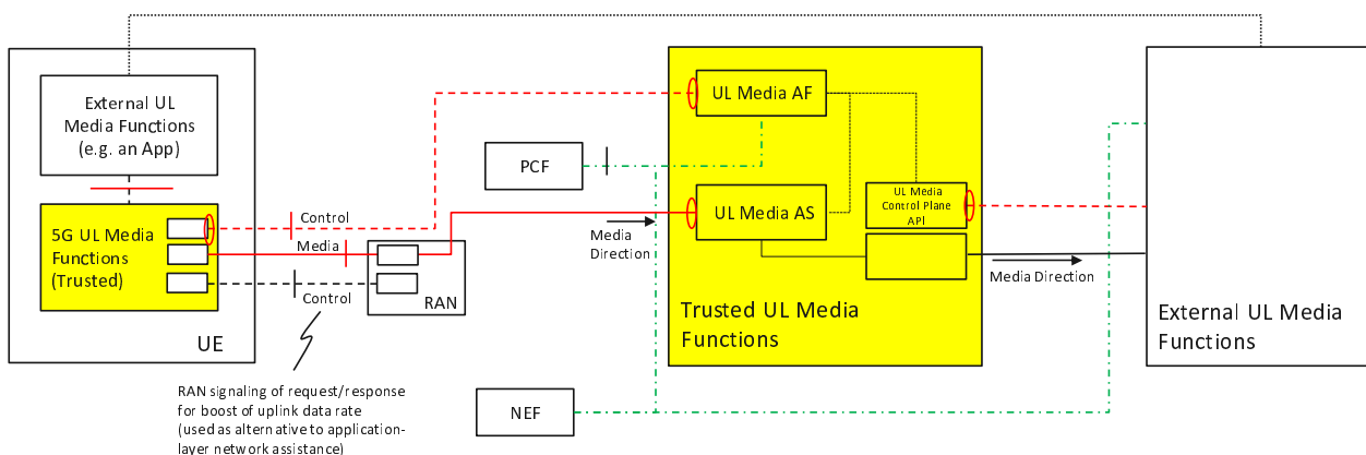
Figure 6.7-1: RAN Signaling based Uplink Network Assistance
