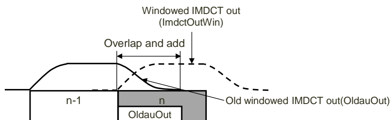
Figure 13: Diagram for describing a windowing of conventional OLA
