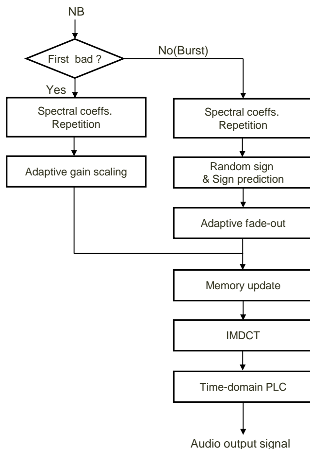
Figure 2: Block diagram for NB PLC for MDCT mode
