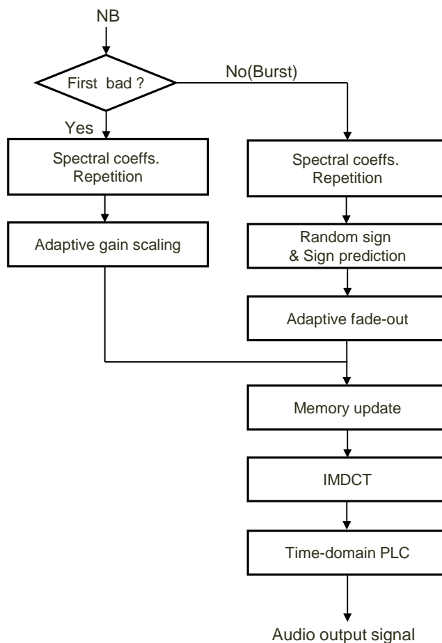
Figure 2: Block diagram for NB PLC for MDCT mode
