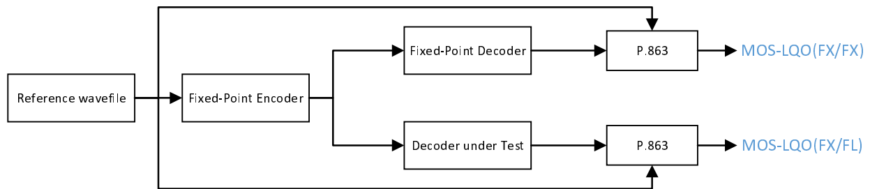
Figure A.5: Flow diagram to obtain the MOS-LQO for 3GPP fixed-point Encoder and floating-point Decoder under Test
