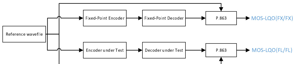
Figure A.4: Flow diagram to obtain the MOS-LQO for floating-point Encoder under Test and floating-point Decoder under Test
