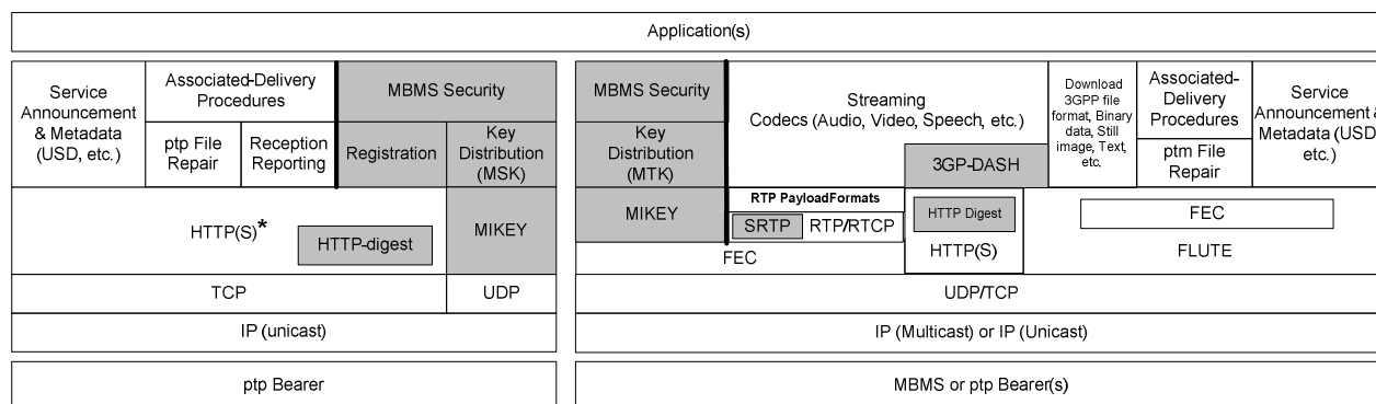
Figure 9: Protocol stack view of the MBMS User Services for Streaming and Download Delivery
