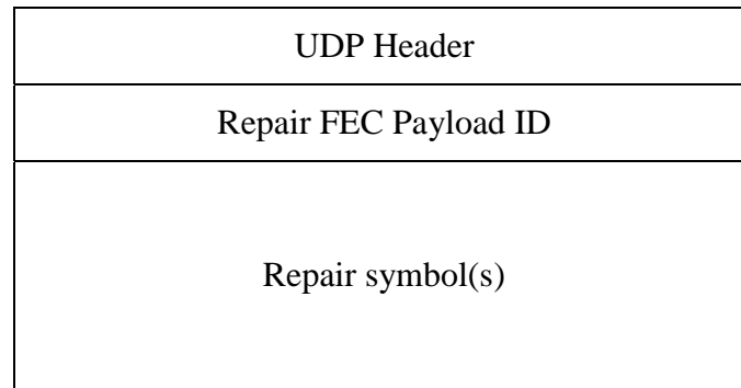
Figure 13: Payload structure for FEC repair packets
