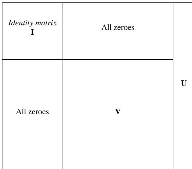
Figure B.2.2-1 – Submatrices of \mathbf{A} in the first phase
