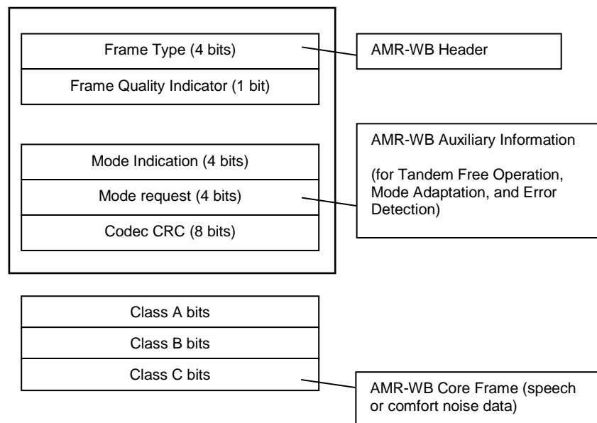
Figure 1. Generic AMR-WB frame structure
