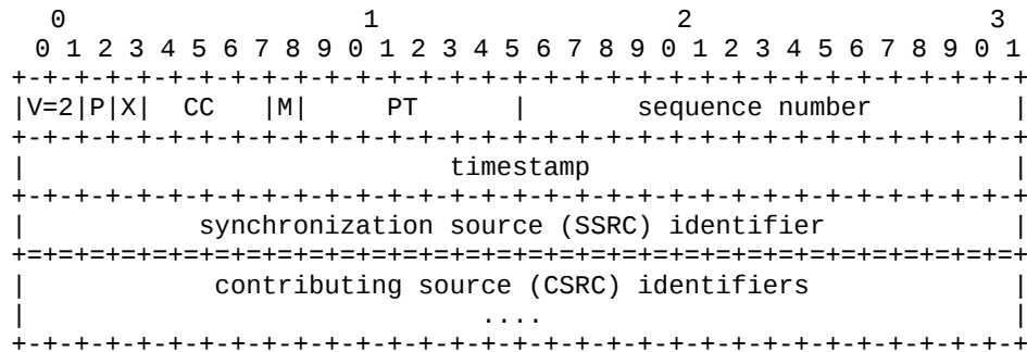
Figure 7-2: RTP HEADER
