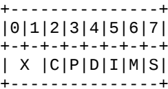
Figure 5-3: DIMS Unit header
