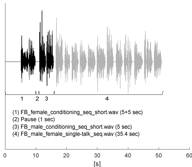
Figure 15a6 Downlink test signal
