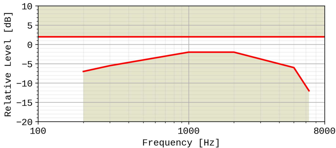
Figure 14b2: Electrical interface receiving sensitivity/frequency mask
