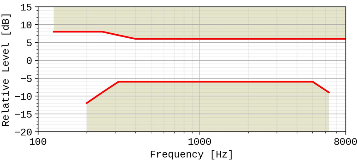
Figure 12: Desktop and vehicle-mounted hands-free receiving sensitivity/frequency mask
