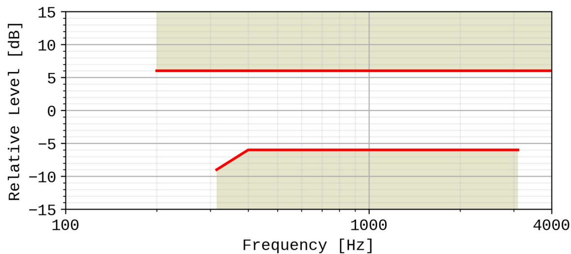
Figure 4: Desktop and vehicle-mounted receiving sensitivity/frequency mask
