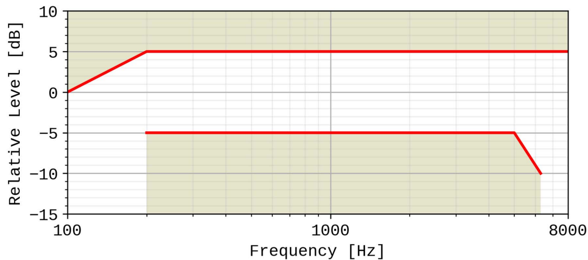
Figure 11: Desktop and vehicle-mounted hands-free sending sensitivity/frequency mask
