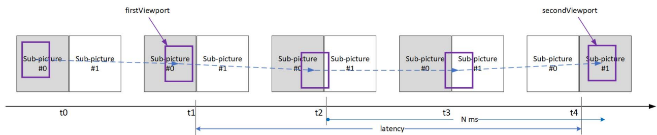
Figure D.1-4: Comparable quality viewport switching latency measurement example
