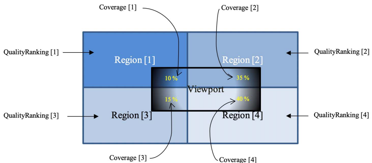
Figure D.1-1: An example of a viewport covered by four quality ranking 2D region
