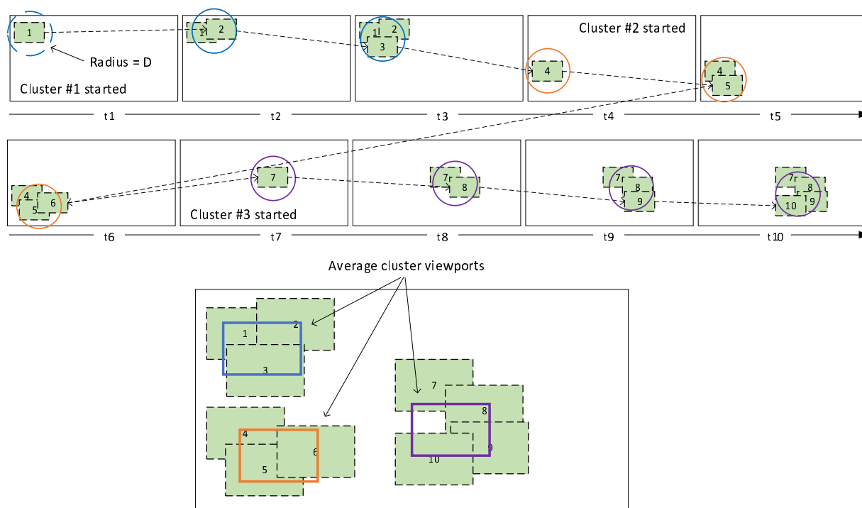
Figure D.2-1: Clustering example
