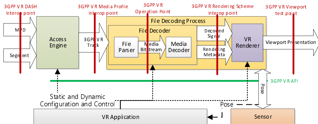
Figure 4.4-1: Interoperability aspects for 3GPP VR Profiles
