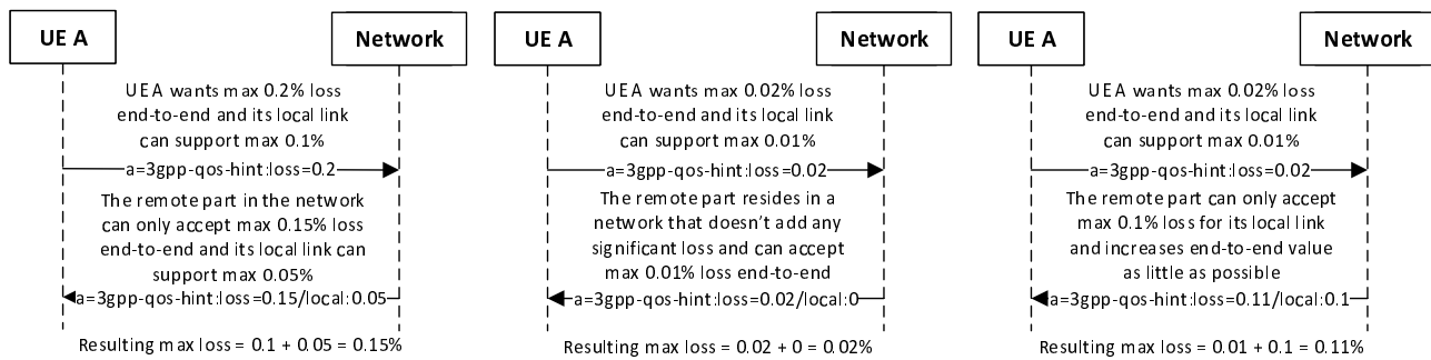
Figure 6.2.7.4.4-2 Illustration of 3gpp-qos-hint "loss" UE-to-Network offer/answer
