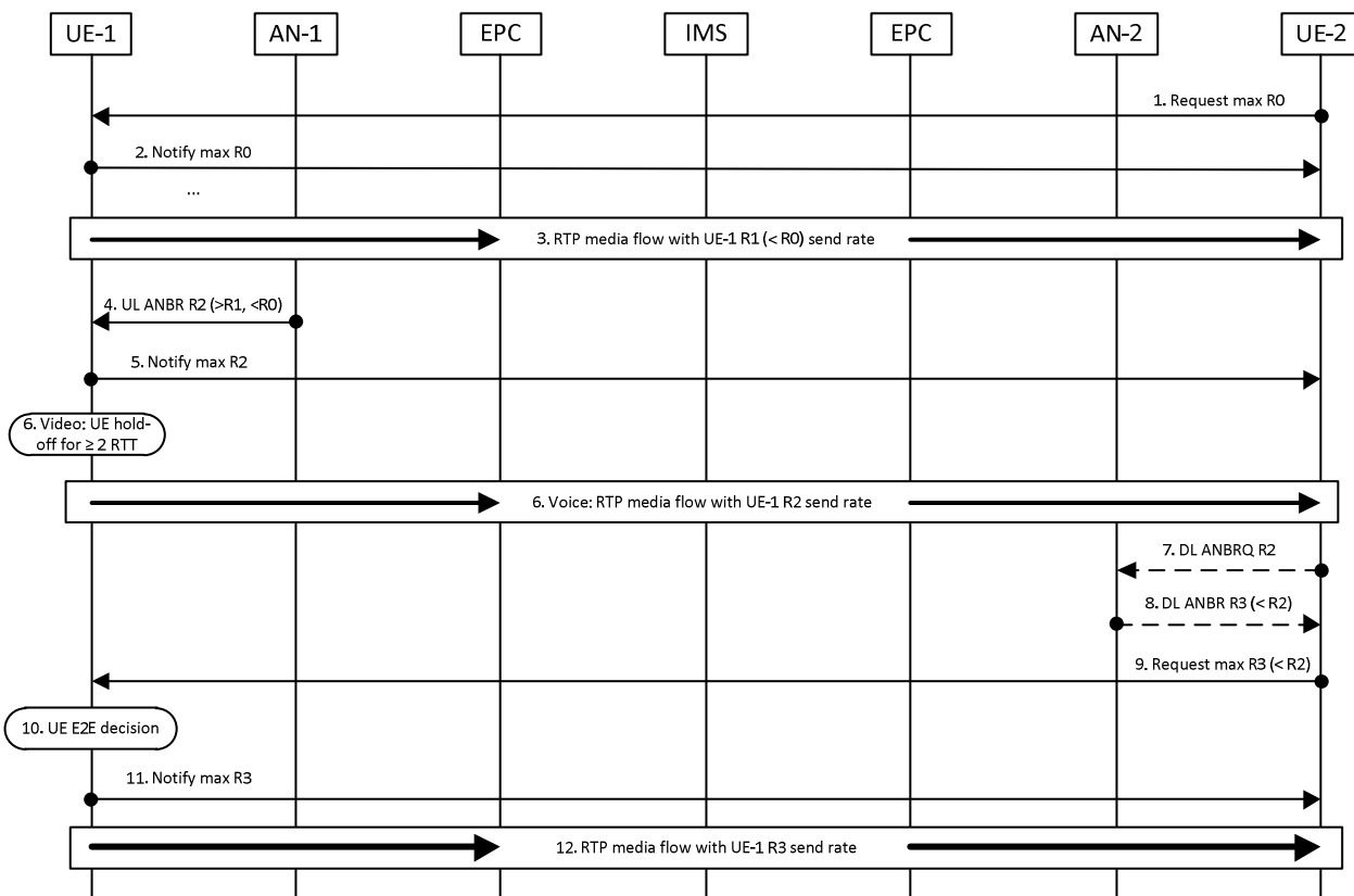
Figure 10.7-2 Uplink bitrate increase based on ANBR
