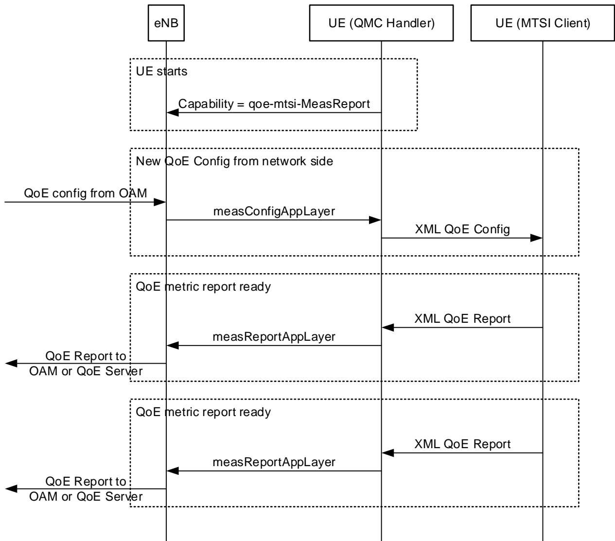
Figure 16.5.1-2: Example signalling diagram for LTE
