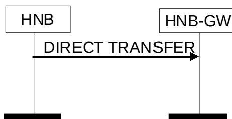
Figure 8.3.3-1: Direct Transfer procedure – successful operation
