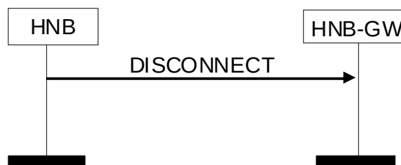
Figure 8.4.2-1: Disconnect procedure
