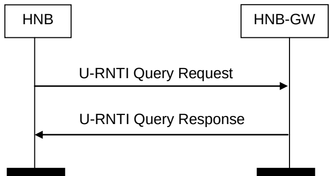
Figure 8.12.2-1: U-RNTI Query procedure: Successful Operation
