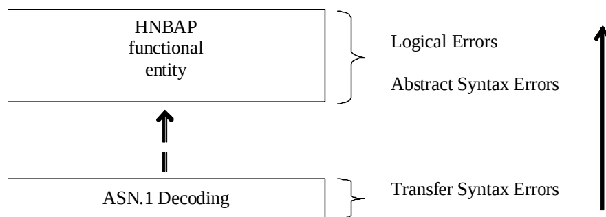
Figure 10.1-1: Protocol Errors in HNBAP
