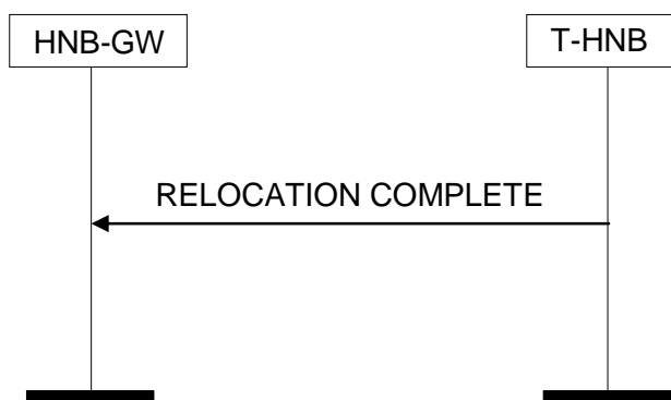
Figure 8.11.2-1: Relocation Complete procedure. Successful operation.
