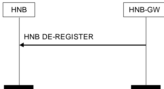
Figure 4: HNB De-register Procedure: Successful Operation
