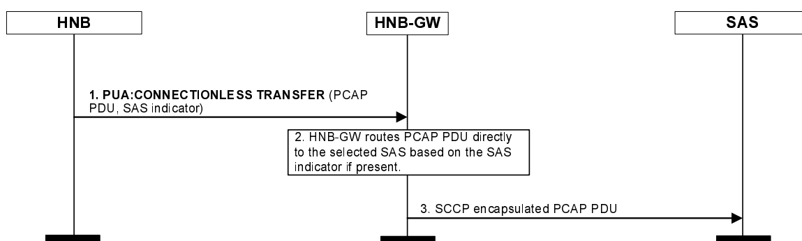
Figure 7.2.2.6.1-1: Connectionless data transfer over luh and luhc connections – HNB initiated.
