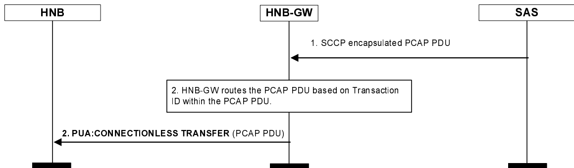
Figure 7.2.2.6.2-1: Connectionless data transfer over luh connections – SAS initiated.
