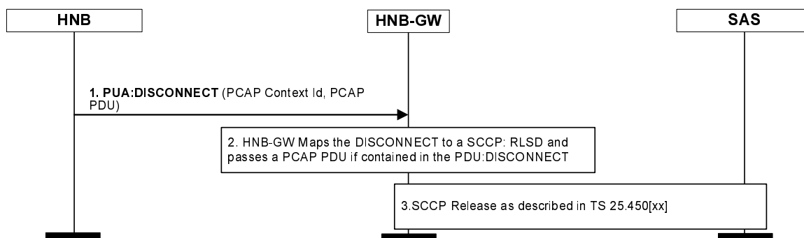
Figure 7.2.2.5-1: Release of established signalling connection over luhc and luh connections – HNB initiated.
