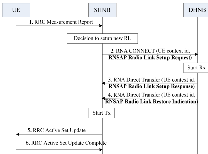
Figure 5.7.3-1: Soft Handover Initiation HNB to HNB.
