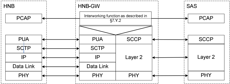
Figure 7.2.1-1: Iupc-luh Interfaces Protocol Stack for connectivity between a HNB and a SAS via the HNB-GW.
