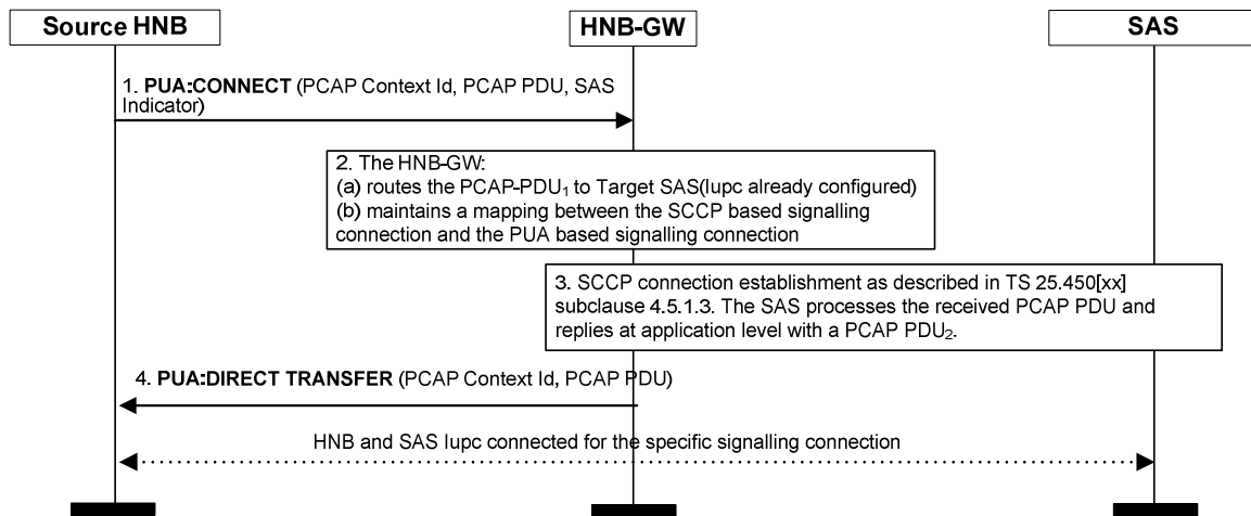
Figure 7.2.2.2-1: Establishment of signalling connection over luhc and luh connections between HNB and SAS via HNB-GW – HNB Initiated.
