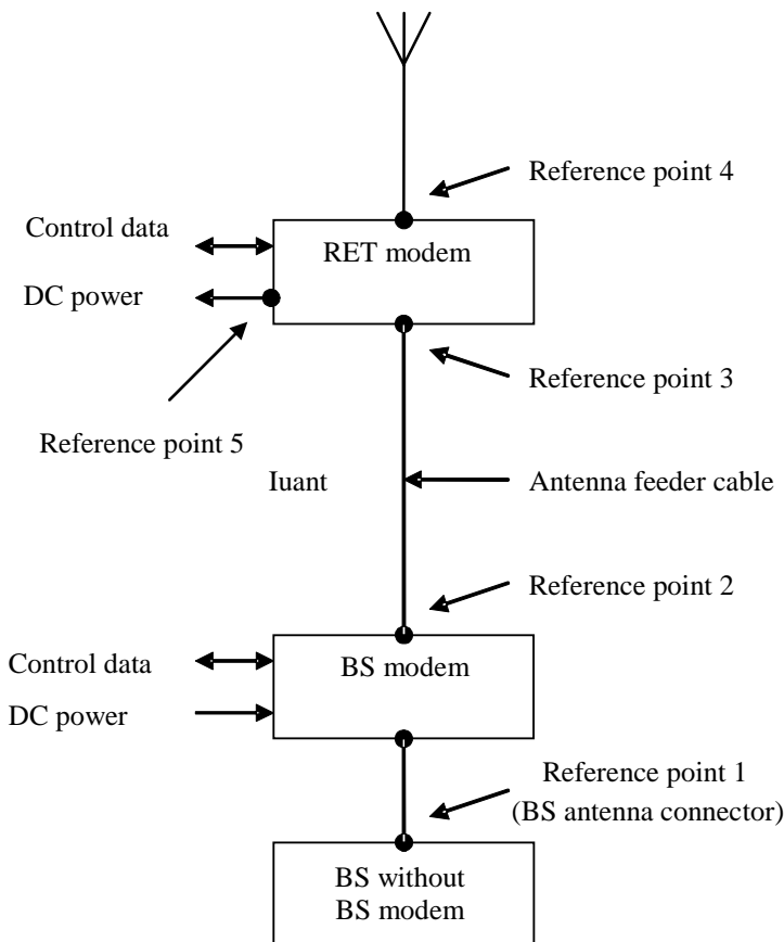
Figure 4.3.1: Modem configuration and modem reference points for a BS without BS modem
