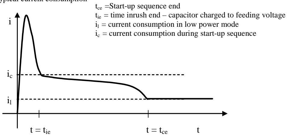
Figure 4.4.3.1 Typical current consumption during the power-up period.
