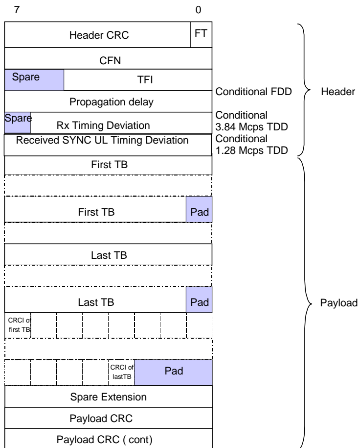
Figure 15: RACH DATA FRAME structure
