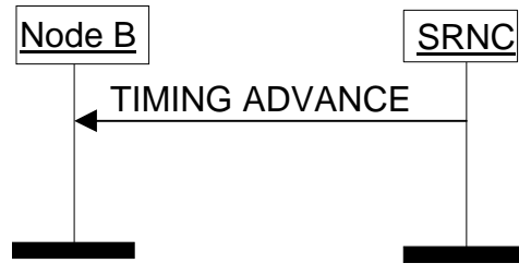
Figure 9A: Timing Advance procedure
