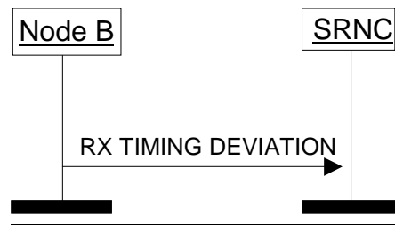
Figure 7: Rx Timing Deviation Measurement procedure
