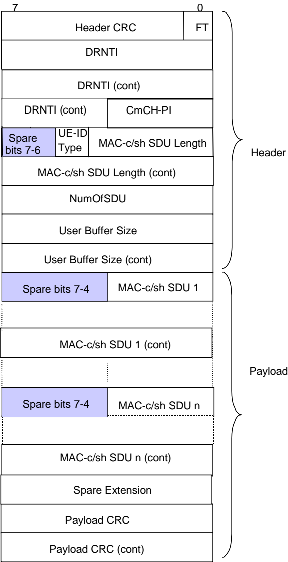
Figure 10: FACH DATA FRAME structure
