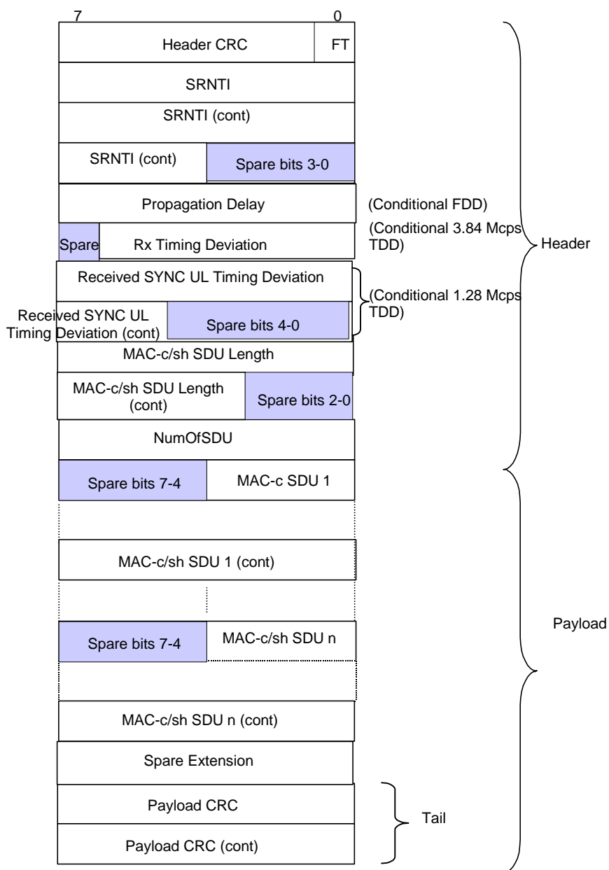
Figure 9: RACH/CPCH[FDD] Data Frame structure
