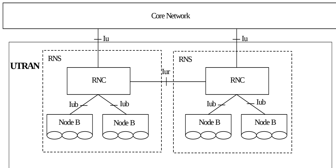
Figure 4: UTRAN Architecture
