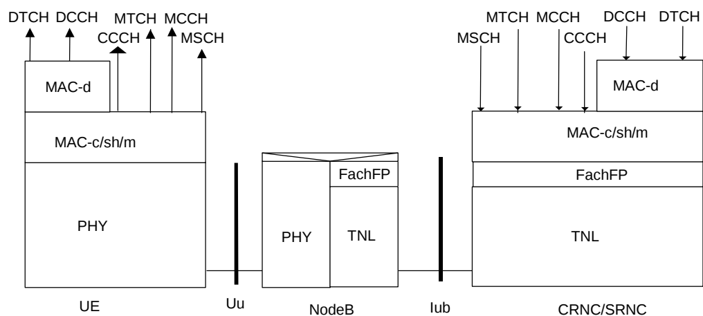
Figure 15: FACH Co-incident Controlling and Serving RNC
