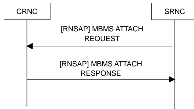
Figure 8.2.11-1: MBMS attach request signalling flow: Successful Operation.
