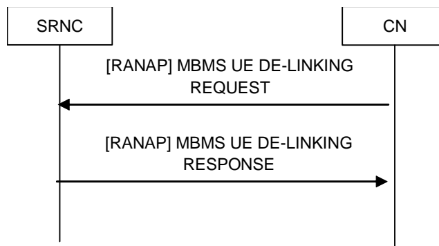
Figure 8.2.9: MBMS UE De-linking signalling flow
