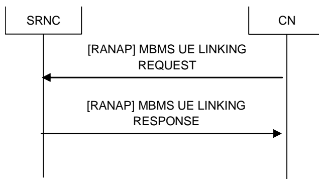
Figure 8.2.8: MBMS UE linking signalling flow
