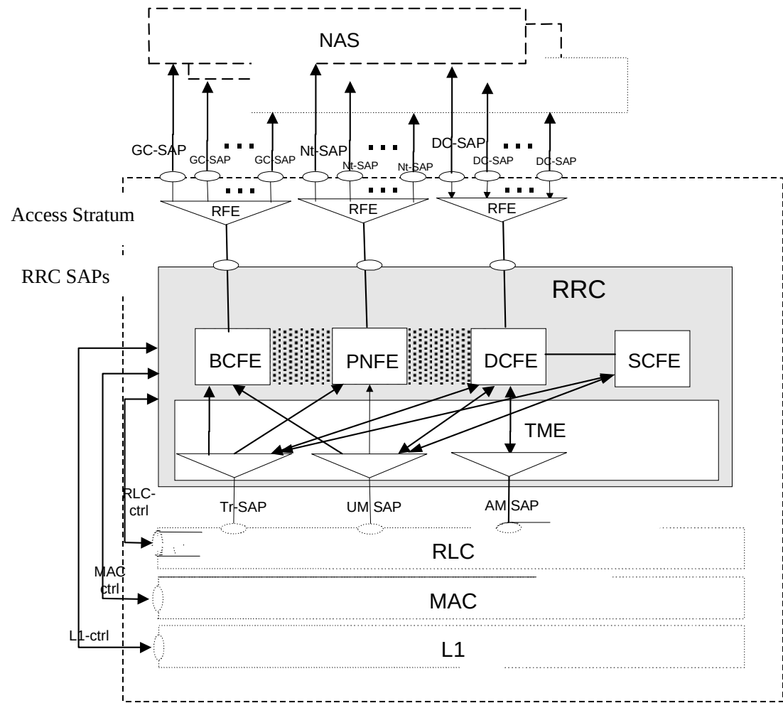
Figure 4.2-1: UE side model of RRC
