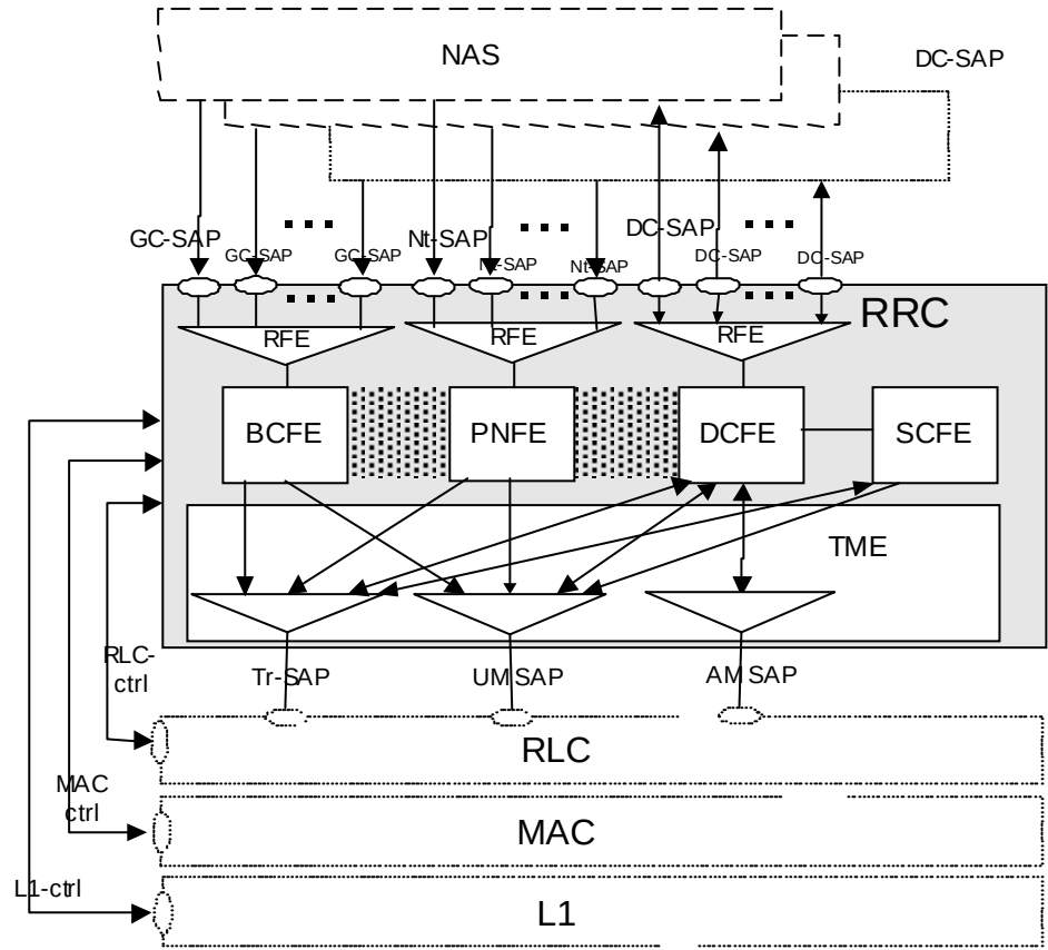
Figure 4.2-3: UTRAN side RRC model (DS-41 System)
