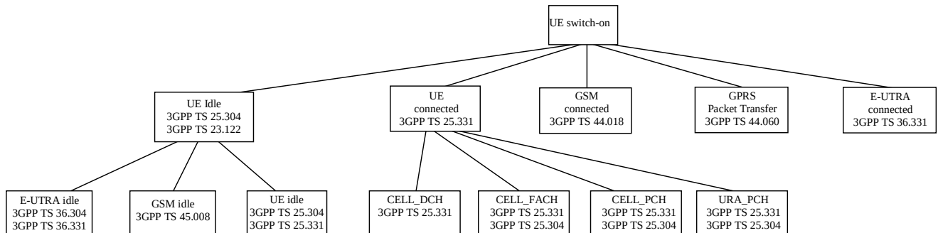
Figure 4.1-1: Mapping of UE state to 3GPP Specifications
