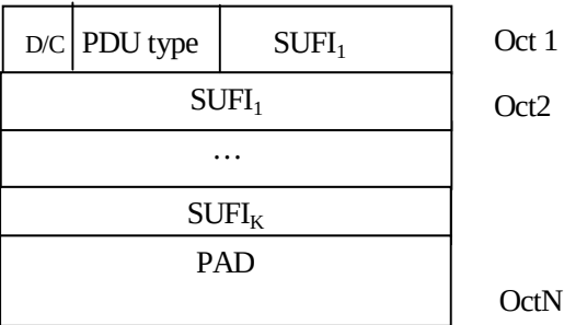
Figure 9.4: STATUS PDU
