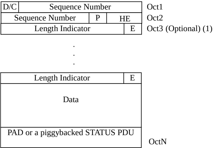
Figure 9.3: AMD PDU
