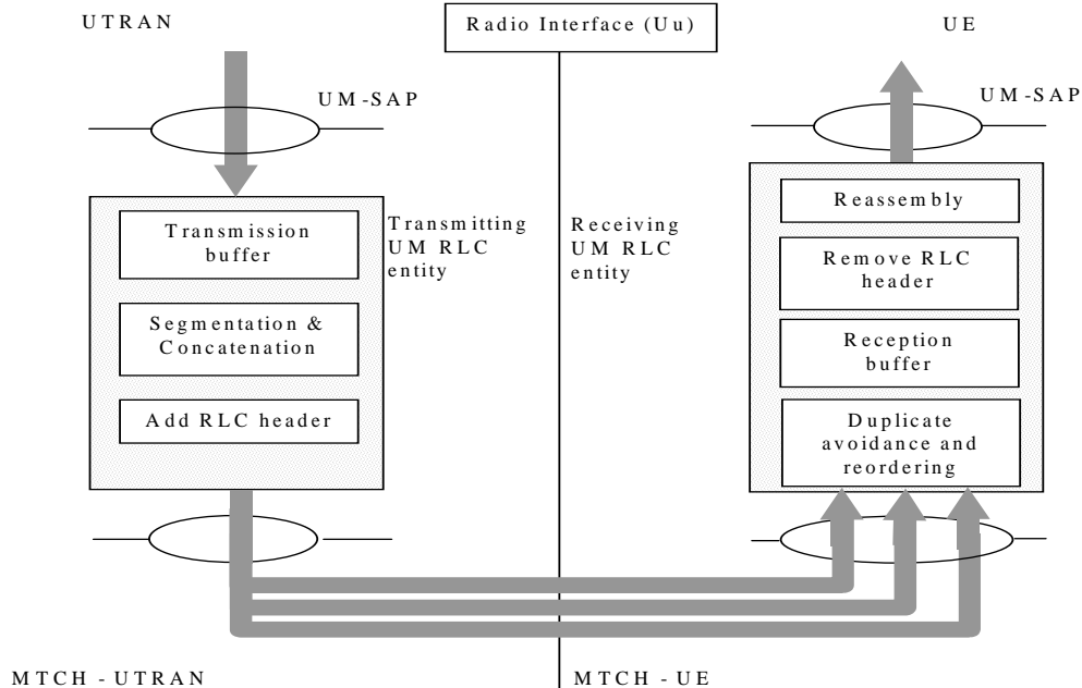
Figure 4.3a below shows the model of two unacknowledged mode peer RLC entities configured for duplicate avoidance and reordering. Because duplicate avoidance and reordering is only specified for MTCH in this release, ciphering/deciphering is omitted.
