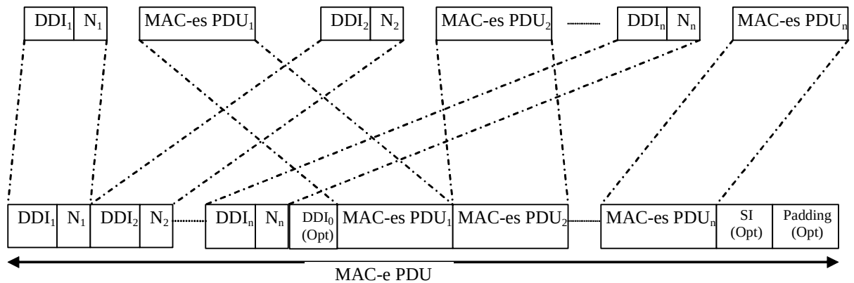
Figure 9.1.5.2a: MAC-e PDU
