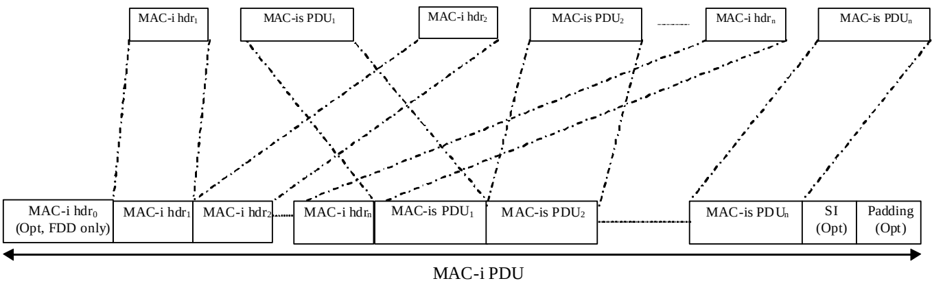
Figure 9.1.5.3 MAC-is PDU.
