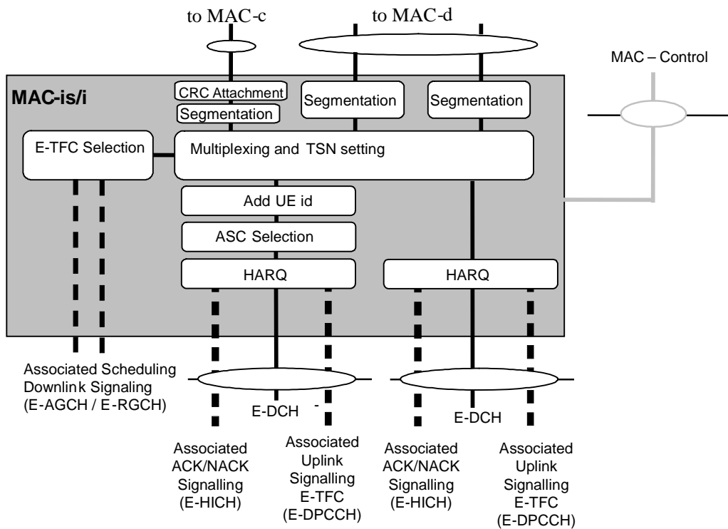
Figure 4.2.3.6-1: UE side MAC architecture / MAC-is/is details (FDD)
