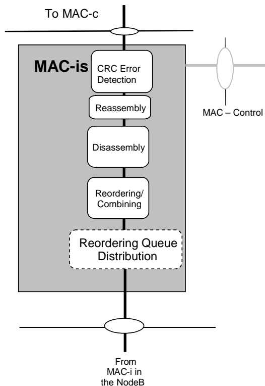
Figure 4.2.4.7-3: UTRAN side MAC architecture / MAC-is details (for CCCH transmission, FDD and 1.28 Mcps TDD only)
