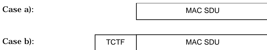
Figure 9.2.1.2.1: MAC PDU formats for BCCH
