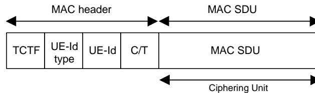
Figure 11.5.1: Cipherring unit for a MAC PDU
