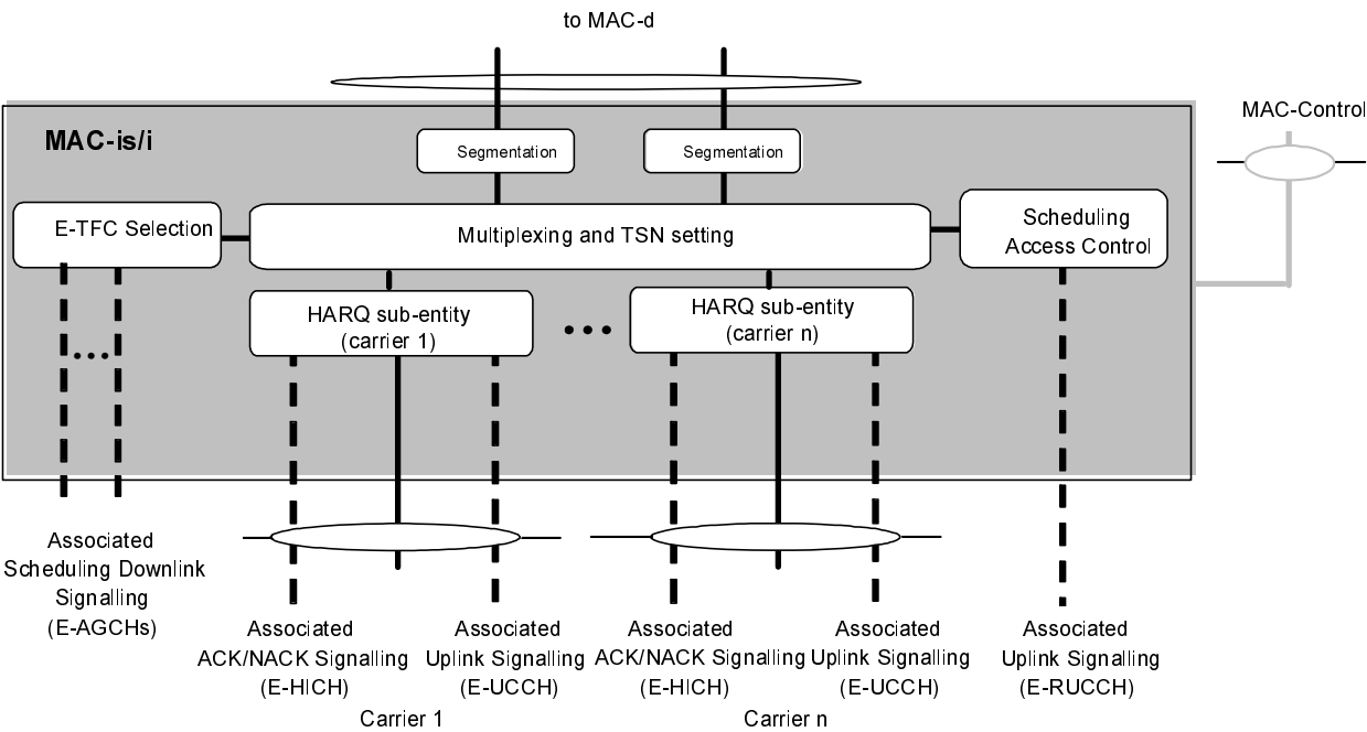
Figure 7.2.6-3a: UE side MAC architecture / MAC-is/i details (1.28 Mcps TDD Multi-Carrier E-DCH operation)
