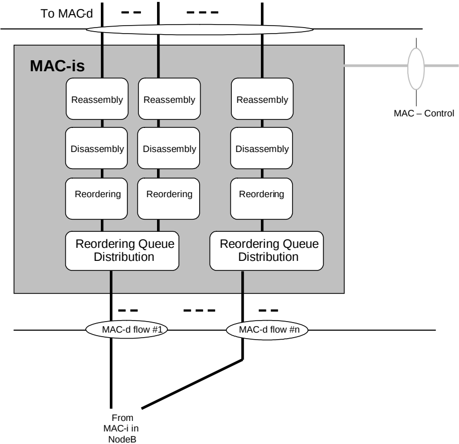
Figure 7.3.7-2: UTRAN side MAC architecture / MAC-is details (for DTCH and DCCH transmission, TDD only)
