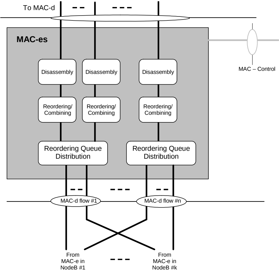
Figure 7.3.5-1: UTRAN side MAC architecture / MAC-es details (SHO case, FDD only)
