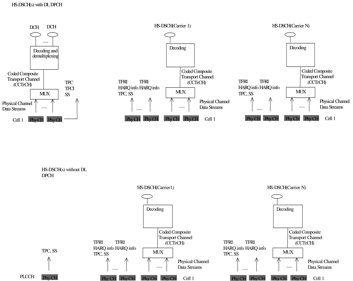
Figure 5.2.2-3: Model of the UE's physical layer (1.28Mcps TDD multi-frequency HS-DSCH operation mode only)
