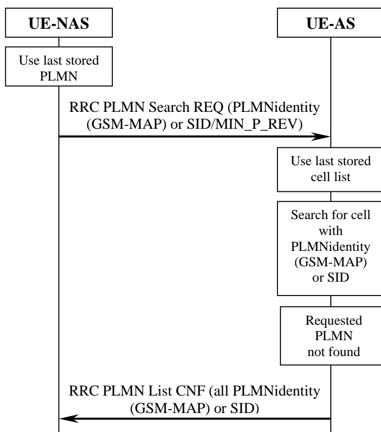
Figure 11: PLMN Selection, automatic mode, selected PLMN not found
