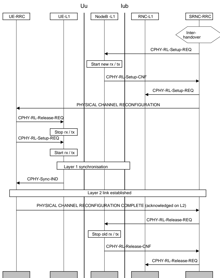
Figure 33: Hard handover
